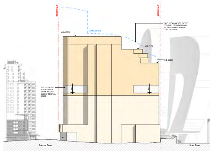
EAST ELEVATION
