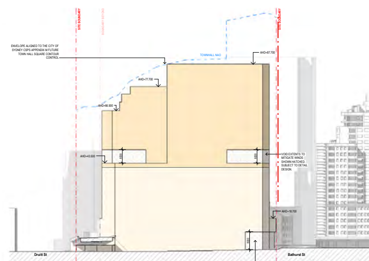
WEST ELEVATION
